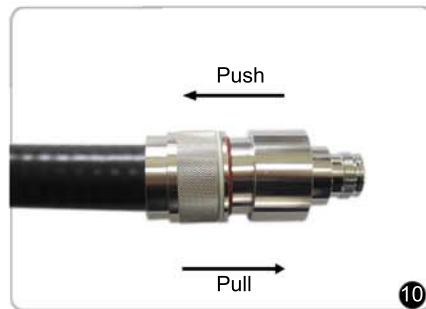
Push the connector onto the cable. Then pull the connector to make sure the connector can not be pulled off.
